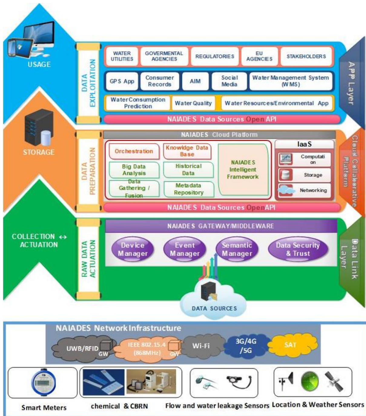
Figure 3: NIADES Overall Architecture.
